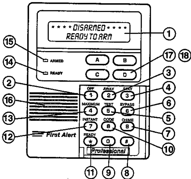
Typical Alpha Console shown above. Fixed-Word Consoles are functionally the same except for screen displays.
